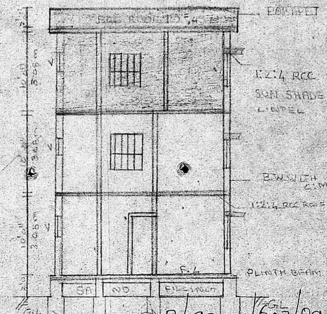
SECTION BB
