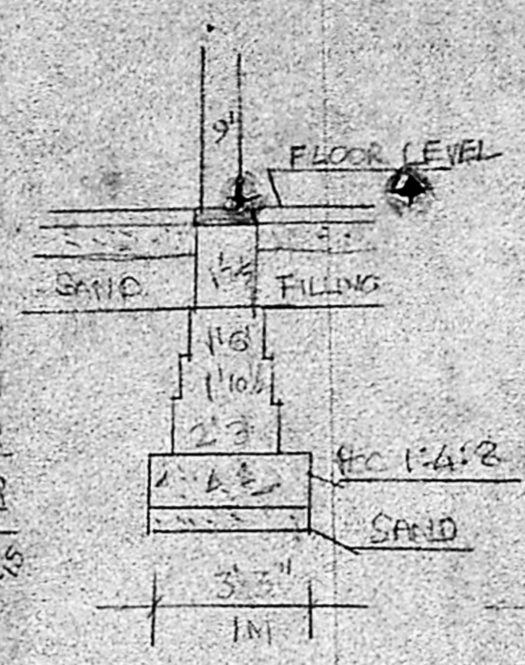
DETAILS - FOUNDATION
